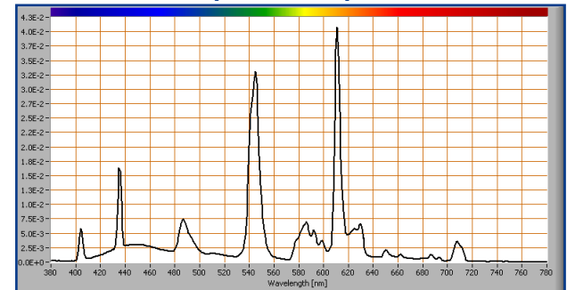
Fluorescent lamp of a competitor, CRI > 95
